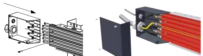
Mounting end feed box to PR7 housing)
