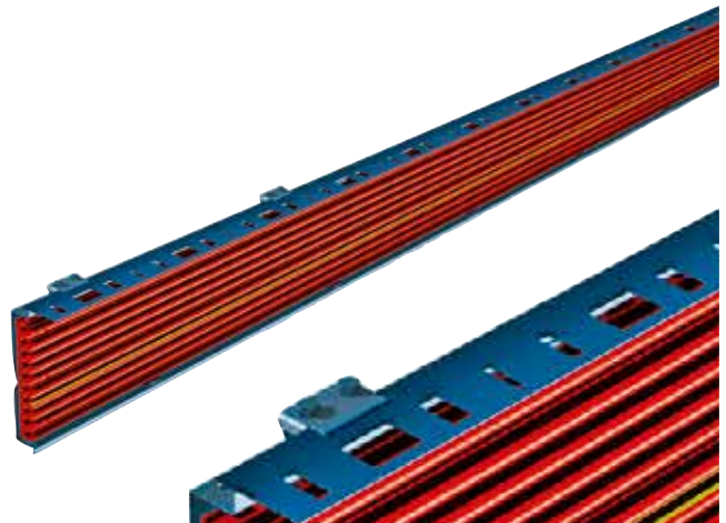
Code tape WCS3 for positioning in combination with a Pro-Ductor system. Mounting of the tape at the bottom of the support profile is also possible.
