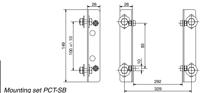
Mounting set PCT-SB
