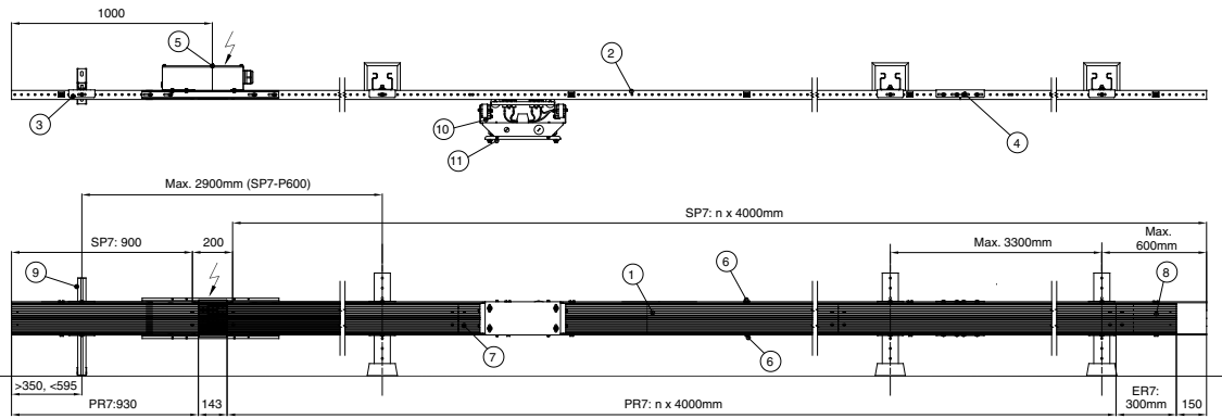
① System type PR7 Line feed as End feed
