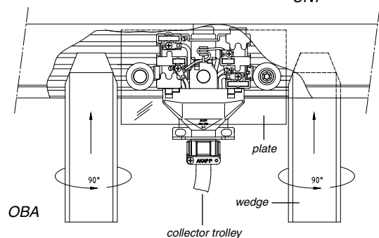
collector trolley
