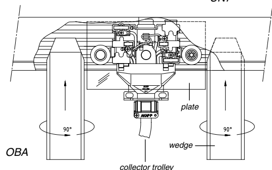
collector trolley
