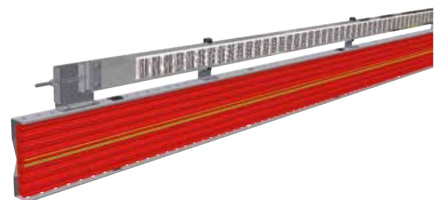
Example of a Pro-Ductor system with positioning by means of barcode strip.
