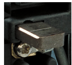
Visual inspection of carbon brushes is rather simple due to the markings as applied.
