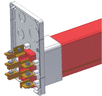
EB40 (opened)
