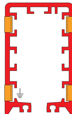
Click-Ductor type RC7-4..
