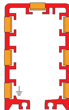
Click-Ductor type RC7-7..
