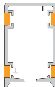
Click-Ductor type RC4-4..
