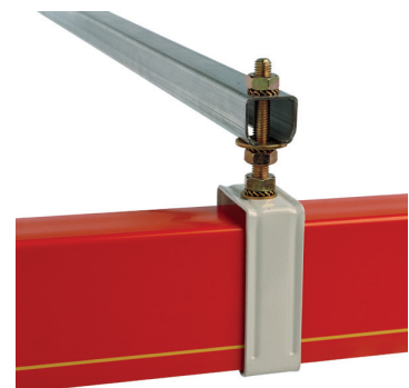
The AKAPP support brackets are of the type 'universal fitting' and easy to position and adjust!
