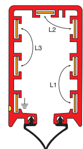
Housing RC7, standard 7-poles, parallel conductors
