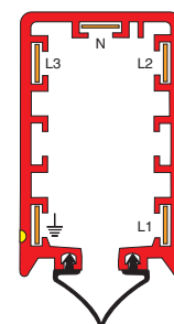
Housing RC7, 5-poles (available only on request)
